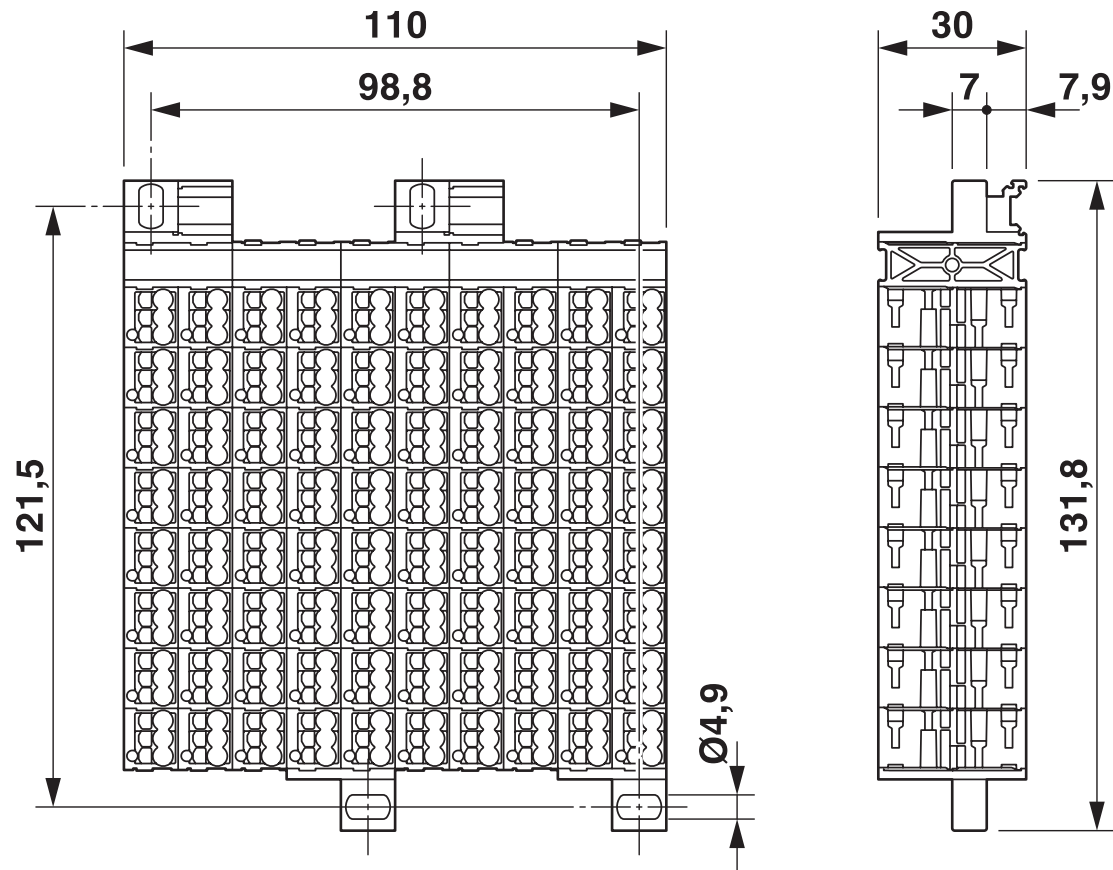
Dimensional drawing
