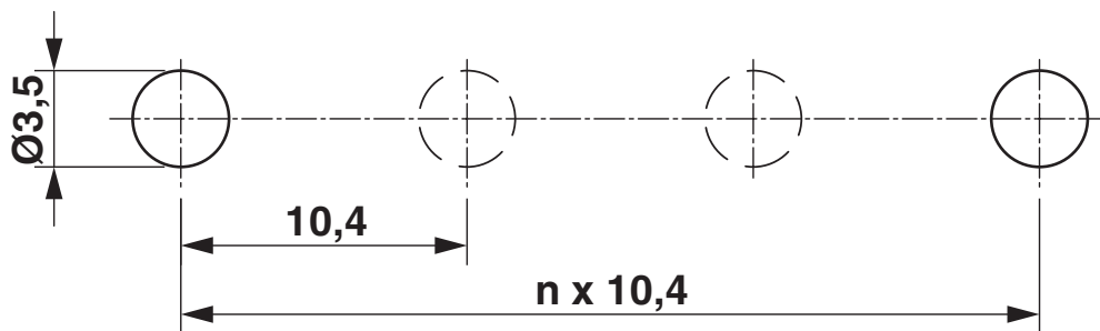
Dimensional drawing
