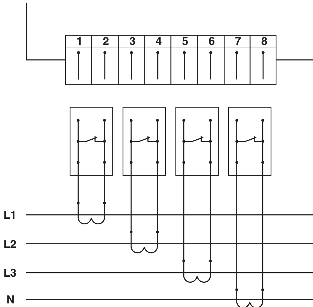
Circuit diagram
