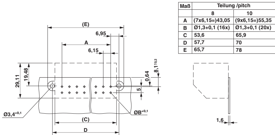
Dimensional drawing
